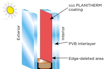
Insulating glass unit with laminated SGG PLANITHERM (coating on face 3)
