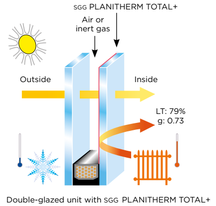
Double-glazed unit with SGG PLANITHERM TOTAL+
